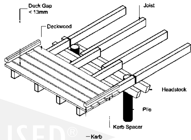
Fig 24 Normal deck system.
