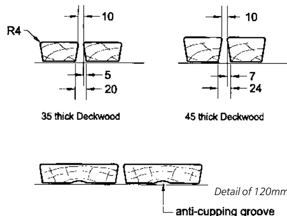
Fig 25 Simplified drawings of OSA's Patented Deckwood profile
