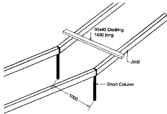
Fig 23 Low profile deck system
