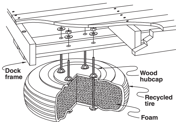
Figure 7—A cross section of a foam-filled tire.
