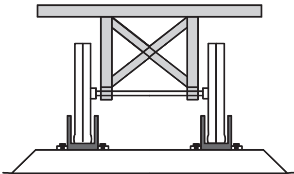
Figure 26—Using deep U-shaped rail channels helps keep the trolley on the tracks. The drawback to this system is that debris accumulates in the channels, causing the trolley to become stuck or derailed.
