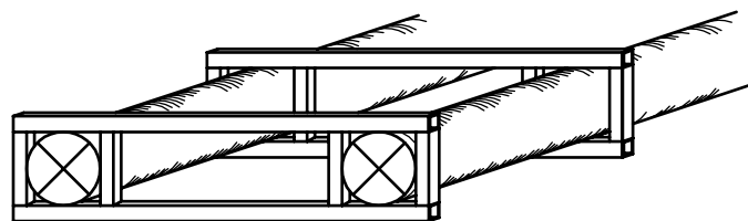
Figure 5—Steel tubing should be framed for adequate structural integrity.
