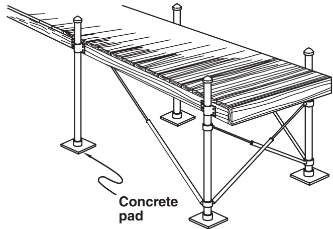
Figure 13—A drawing of a dock supported by pipe legs. Pipe-leg-based structures are one of the most environmentally gentle ways of crossing wet areas.
